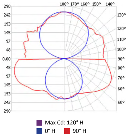
Polar Candela for 18W 3' T12 Tube
